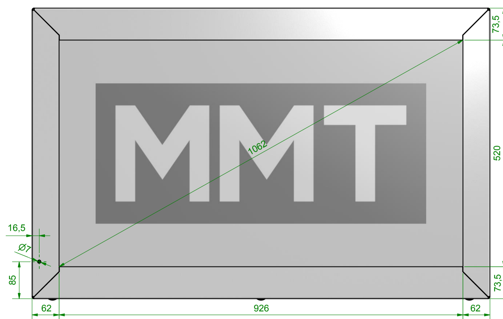
Front View 1:5
