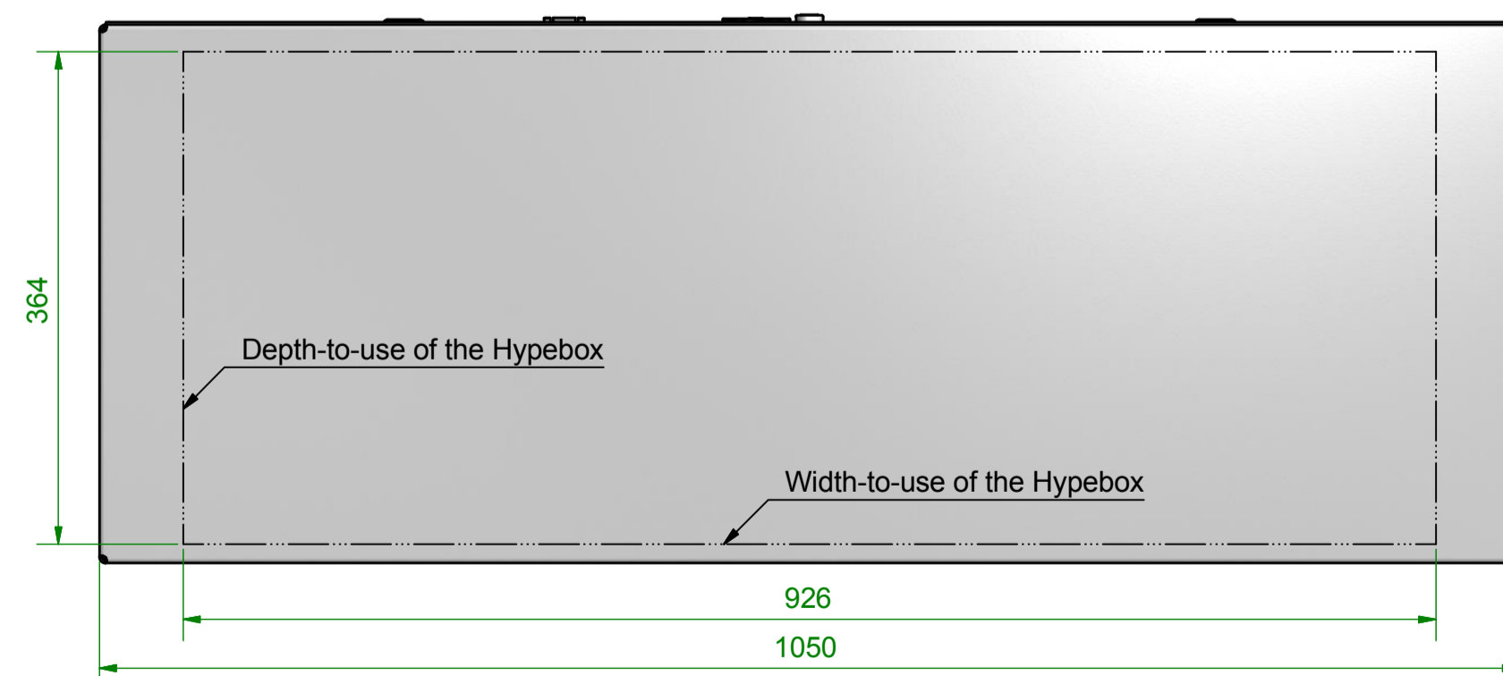
Top View 1:5
