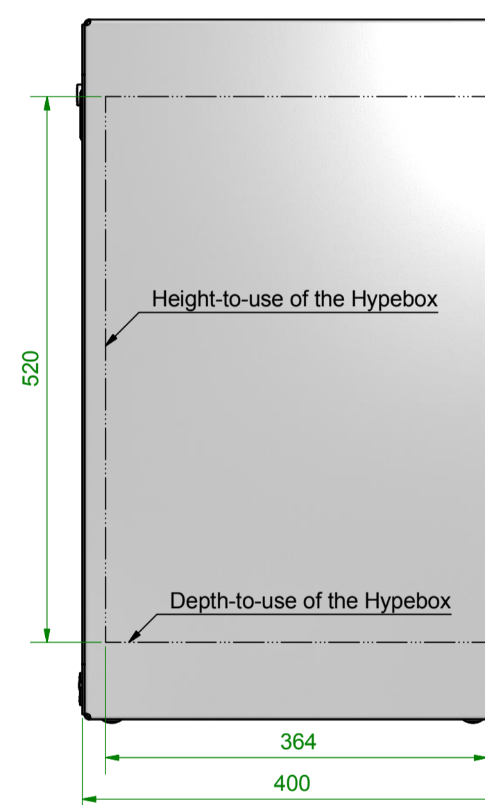
Lefthand View 1:5
